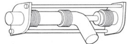
| Tip MPB - Pressure Balanced Expansion Joint | sketch
