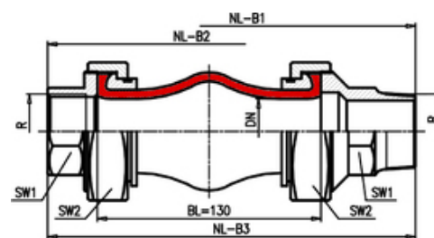
| Tip B3 (filet interior-exterior) - Compensator cauciuc | dimensionare
